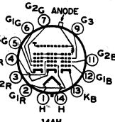
14AH ANODE = G_4 + G_5 + CL + R FOCUSING ELECTRODE = G_3
