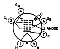
8KW ANODE = G_3 + G_5 + CL FOCUSING ELECTRODE = G_4
